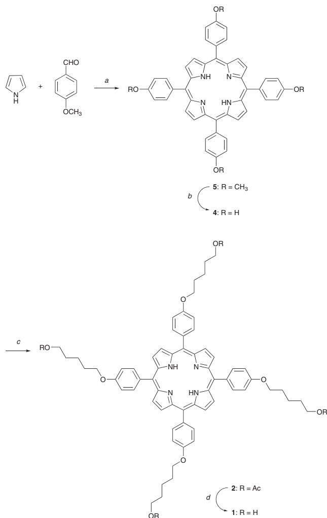
Scheme 2. Synthesis of tetrahydroxyporphyrin 1 . Reagents and conditions: a propionic acid, reflux; b pyridinium hydrochloride, 22 h, reflux; c \text{Br}(\text{CH}_2)_5\text{OCOCH}_3 , \text{K}_2\text{CO}_3 , 18-crown-6, 60 °C, 2 h; d \text{NaOCH}_3 , THF, reflux 3 h.
