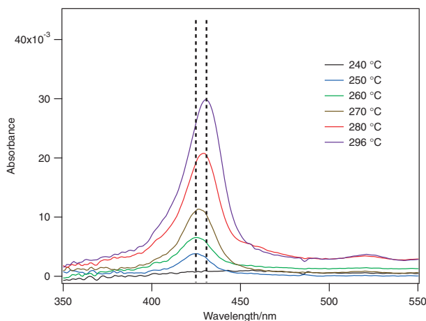
Figure 10. UV-visible spectra of ether porphyrin 3 spin-coated on silica glass followed by heat treatment at the designated temperatures between 240 and 296 °C for 10 min. The absorption maximum heated at 296 °C was 430 nm while that heated at 250 °C was 426 nm.
