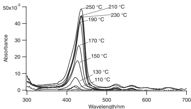
Figure 6. UV-visible spectra of porphyrin alcohol 1 spin-coated on silicate glass followed by heat treatment at 80, 90, 100, 110, 130, 150, 170, 190, 210, 230, and 250 °C for 10 min. The absorption maximum at 130 °C was 421 nm while that at 250 °C was 436 nm.
