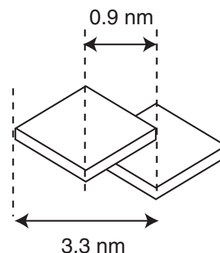
Figure 8. Schematic representation of a dimer structure deduced from the UV–visible spectral shift for an aggregate of 1 . The molecule of 1 is shown as a square. The distance between the centers of 1 was calculated to be 0.9 nm on the basis of Kasha's theory.
