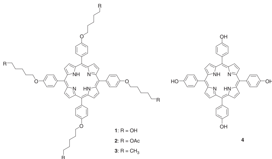
Chart 1. Porphyrin derivatives 1, 2, 3, and 4.
