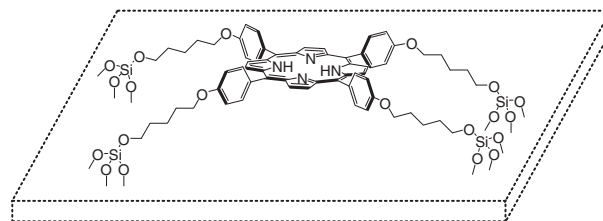
Figure 4. Schematic representation of 1 adsorbed onto silica surface.
