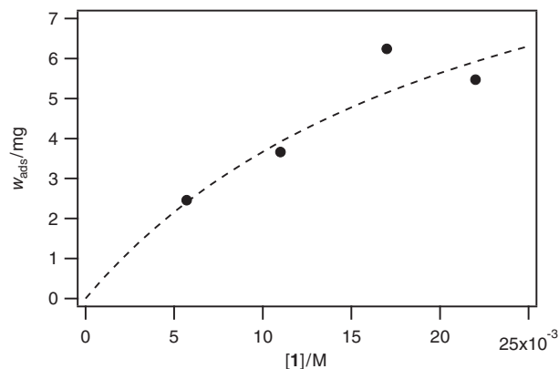
Figure 3. Plot of adsorbed 1 onto 50 mg of CARiACT against the concentration of 1 in pyridine. Data taken from Runs 6–9 in Table 1. The dotted line is drawn on the basis of the Langmuir isotherm: w_{\text{ads}} = w_{\text{max}}a[1]/(1 + a[1]) .
