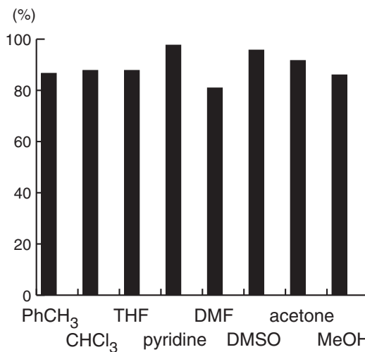
Figure 9. Absorbance of the Soret band of 1 on silicate glass after immersion in various organic solvents for 5 h at 25 °C and washing with pyridine.
