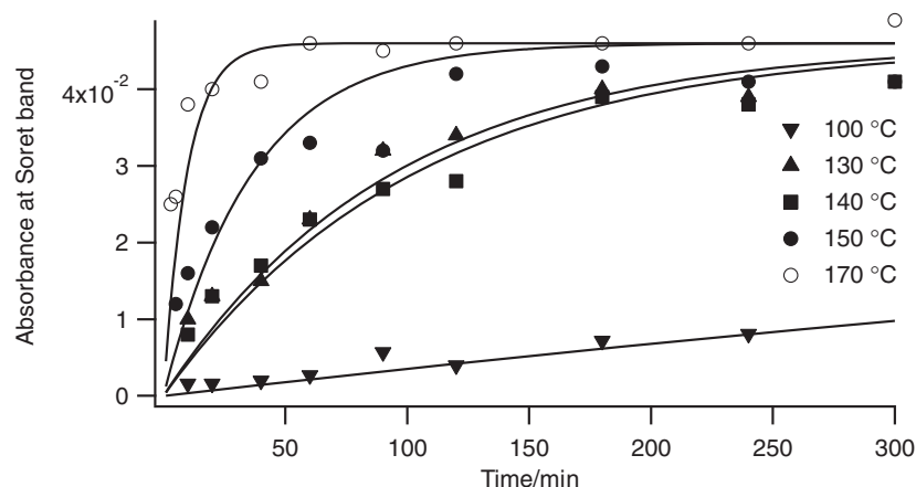
Figure 7. Plot of absorbance of the absorption maxima of the Soret band at 423–436 nm of a silicate glass spin-coated with 1 and heated at 100, 130, 140, 150, and 170 °C against heating periods. The curve obtained by fit the data to Langmuir adsorption rate equation: Abs = 0.046(1 - \exp(-kt)) is shown, where k = 0.0008 (100 °C), 0.0106 (130 °C), 0.0097 (140 °C), 0.0274 (150 °C), and 0.104 min -1 (170 °C).
