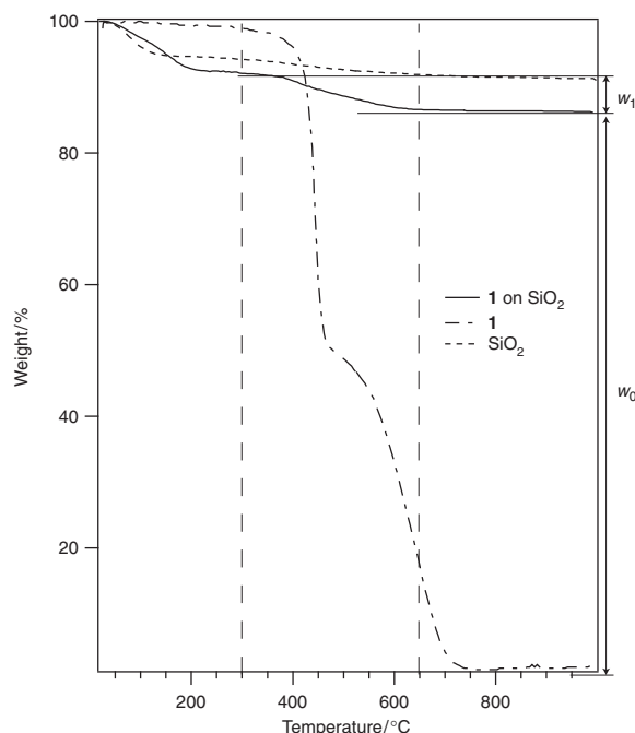
Figure 2. TG traces of 1 adsorbed on the silica gel, 1 , and the silica gel. The sample was heated at a rate of 15 °C \text{min}^{-1} in air. Porphyrin 1 (9 mg) was allowed to react with CARICT (50 mg) at 110 °C in pyridine (0.5 mL). Evaporation of the pyridine, addition of another portion of pyridine, and heating at 110 °C was repeated three times.
