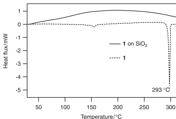
Figure 5. The DSC traces of 1 and the 1 -SiO 2 hybrid.
