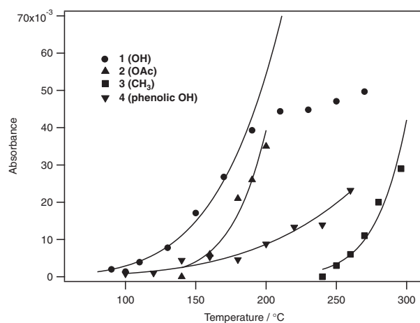
Figure 12. Plot of absorbance of the Soret band against the reaction temperatures for 1 , 2 , 3 , and 4 . The reaction period was 10 min. The curves fit to the Arrhenius equation, Abs = A \exp(-\Delta E / (temp + 273.15)) , are shown. The absorbance of 1 heat-treated above 210 °C was much lower than expected from the Arrhenius equation.
