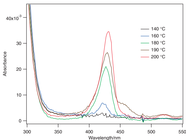
Figure 11. UV-visible spectra of ester porphyrin 2 spin-coated on silica glass followed by heat treatment at the designated temperatures between 140 and 200 °C for 10 min. The absorption maximum heated at 200 °C was 431 nm while that heated at 160 °C was 421 nm.
